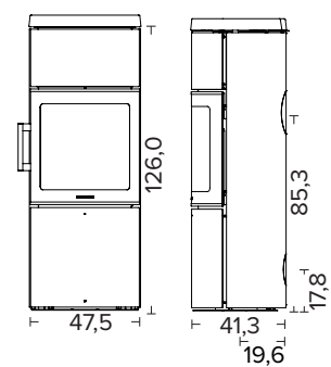
HWAM 3130m Standardgreb
