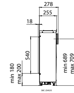
Global 100 BF | 120 BF (P. 85)
