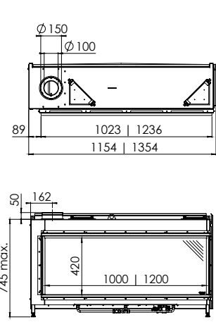
Global 100 BF | 120 BF (P. 85)
